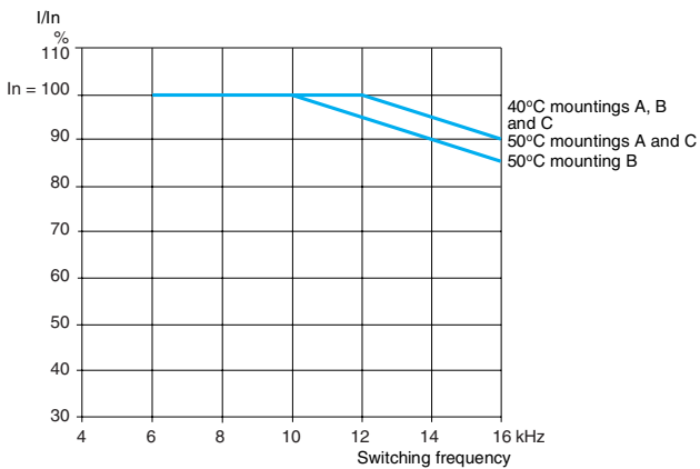
ATV 21HU30M3X
