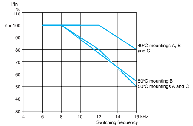
ATV 21HD55N4
