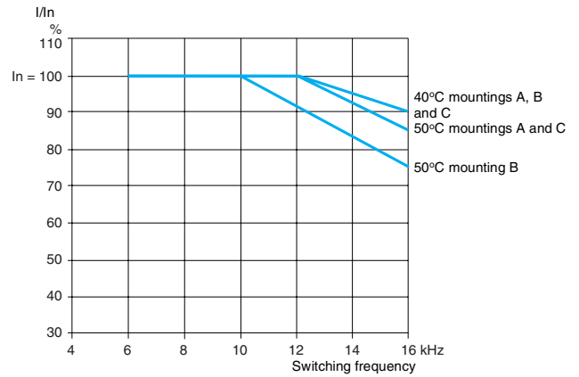
ATV 21HU40N4
