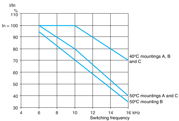
ATV 21HD30N4
