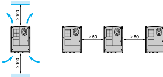
ATV 21W000N4, ATV 21W000N4C
