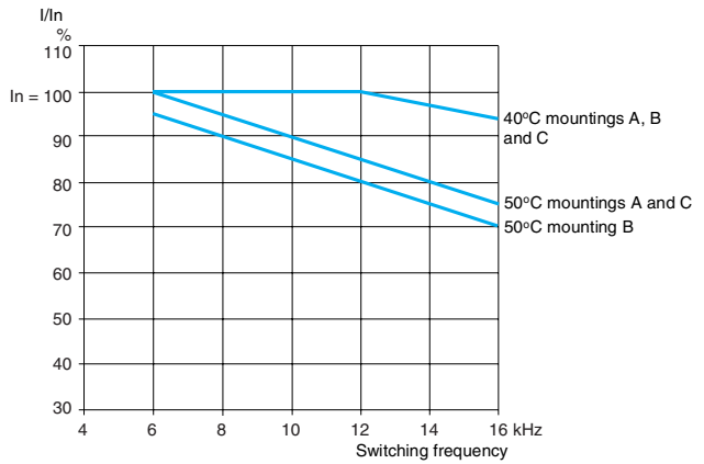
ATV 21HD18M3X
