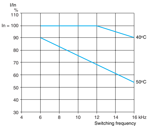
ATV 21W075N4...WU75N4, ATV 21W075N4C...WU75N4C
