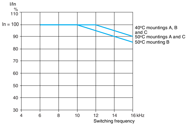
ATV 21H075M3X
