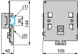
(1) rail (2) Kit
