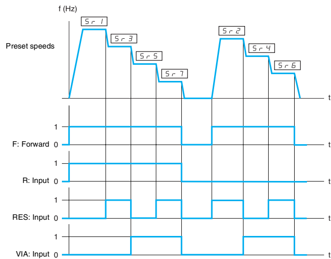
Example of operation with 7 preset speeds
