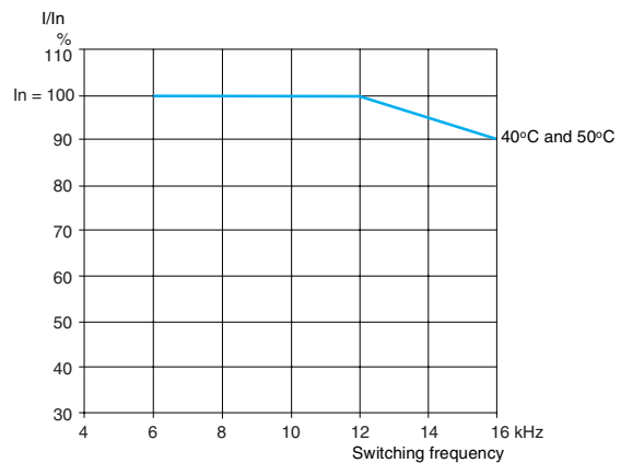
ATV 21WD11N4, ATV 21WD11N4C
