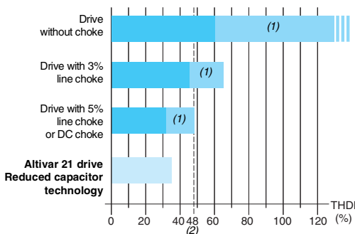
THDI: Total current harmonic distortion (1) Typical use (2) Maximum THDI conforming to standard IEC/EN 61000-3-12
