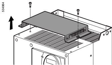
Removing the protective blanking cover for: ATV 21HD22M3X, HD30M3X, ATV 21HD22N4...HD75N4
