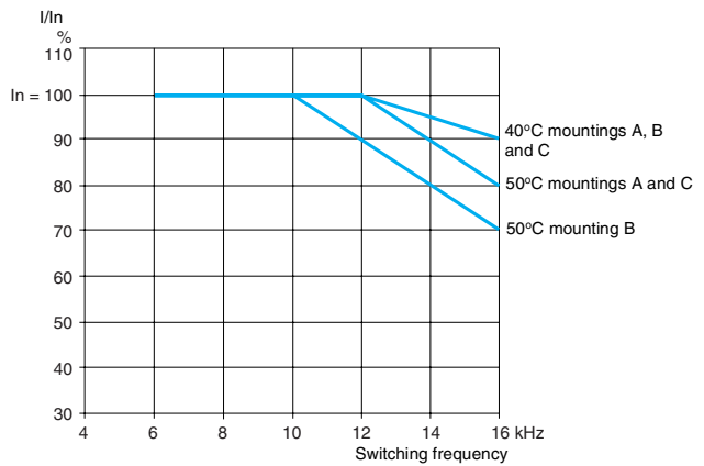
ATV 21HU22N4
