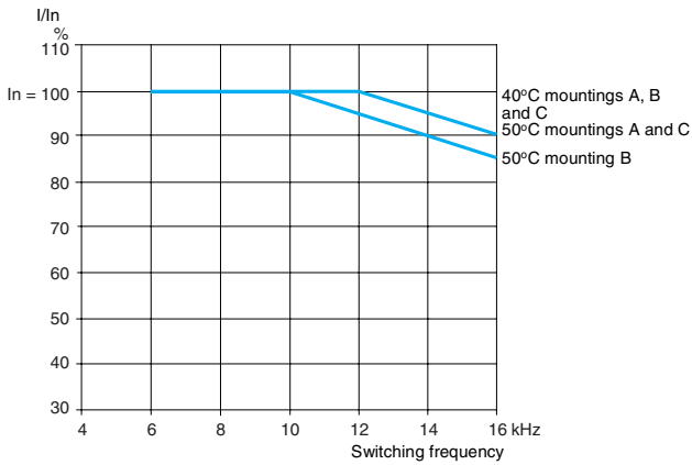
ATV 21HU55M3X...HD15M3X
