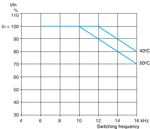
ATV 21WD15N4, ATV 21WD15N4C
