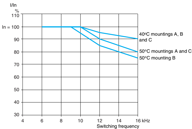
ATV 21HD22M3X
