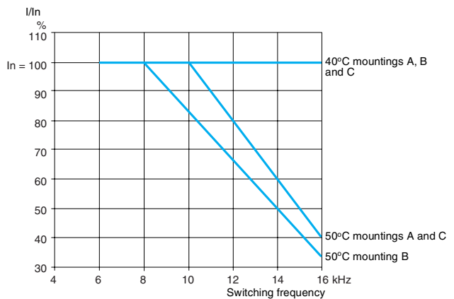
ATV 21HD30M3X
