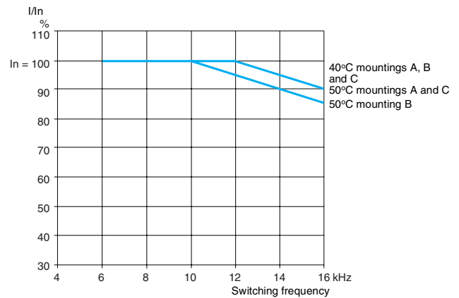
ATV 21HU75N4
