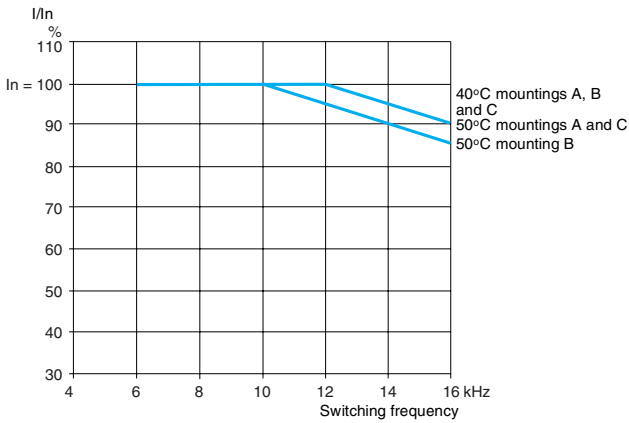
ATV 21HU30N4
